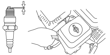
Figure 4-8. Spark Plug
